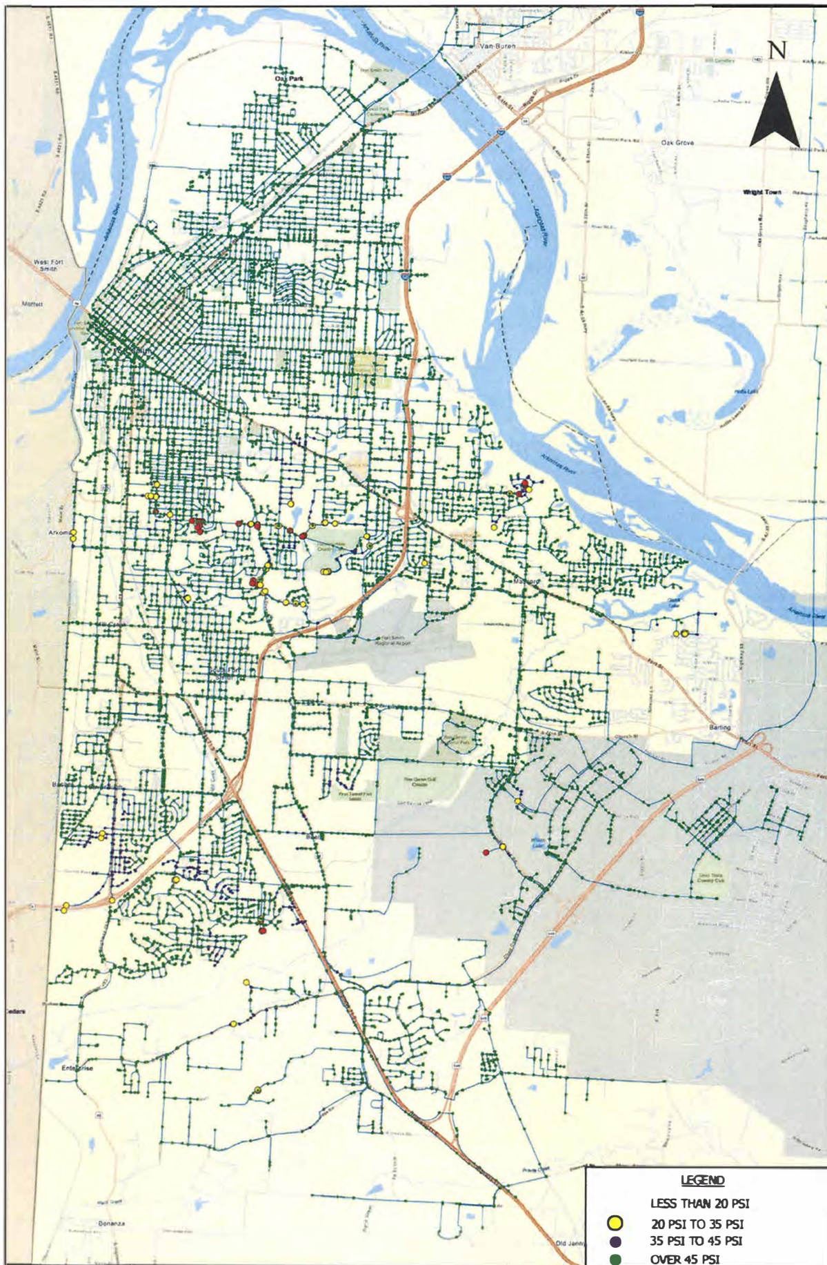
WATER MASTER PLAN - CITY OF FORT SMITH, ARKANSAS FIGURE 9 2031 MDD MINIMUM PRESSURE WITH PROPOSED IMPROVEMENTS
